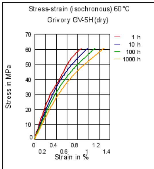
Stress-strain (isochronous) 60°C
