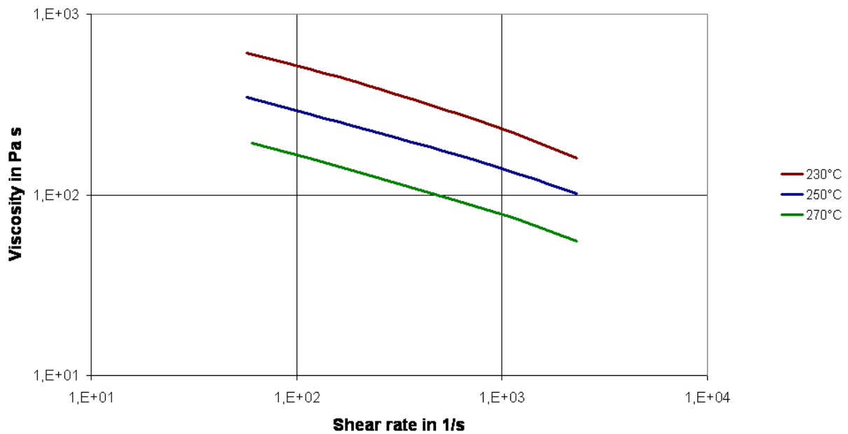
Viscosity-shear rate Technylstar S 60G1 V30
