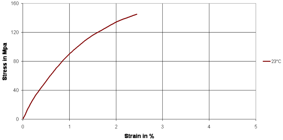
Stress-Strain (dry) Technylstar S 60G1 V30
